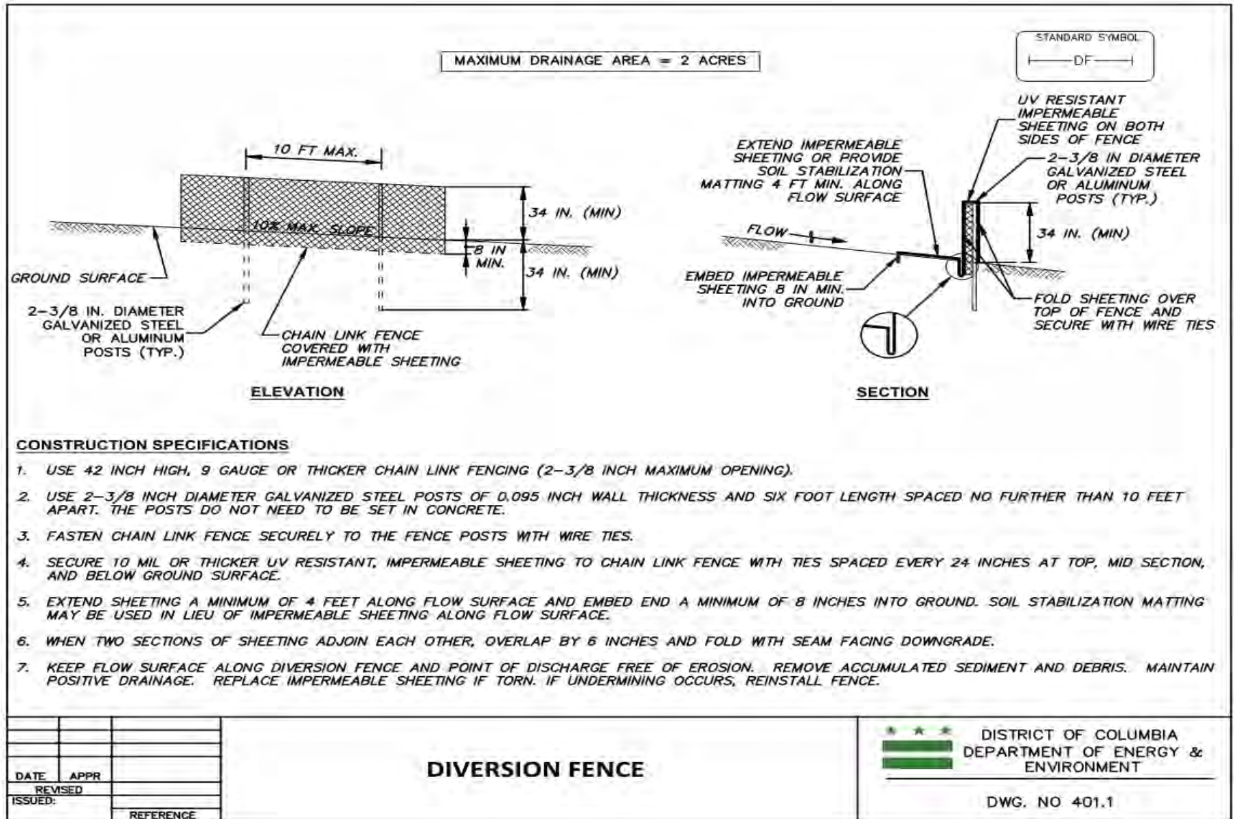
Detail 28 – 401.1 Diversion Fence
