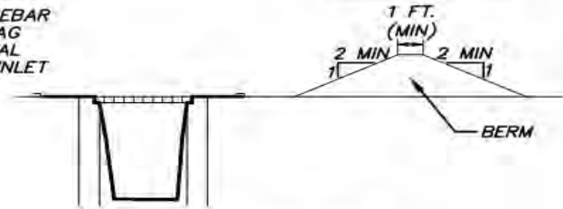
ELEVATION VIEW
