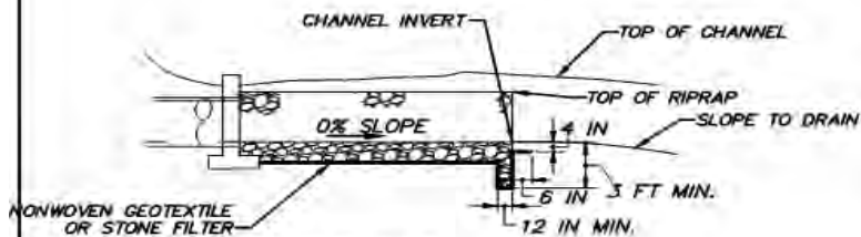
PROFILE
