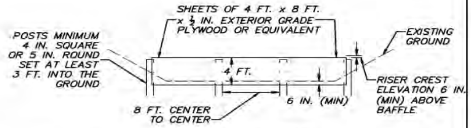
BAFFLE DETAIL
