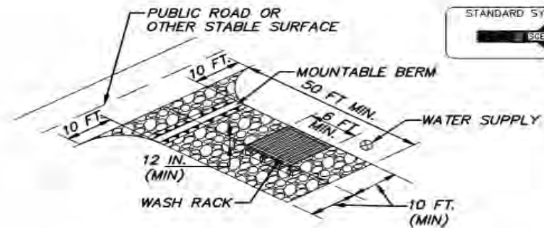
ISOMETRIC VIEW - WASH RACK ALONG SCE
