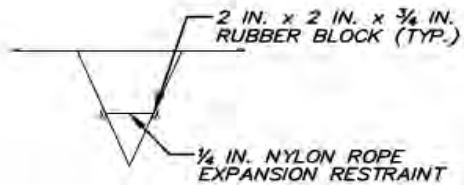
INSTALLATION DETAIL
