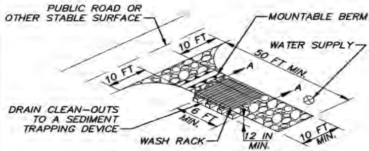
ISOMETRIC VIEW - WASH RACK IN SCE
