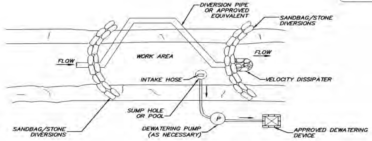
PLAN VIEW
