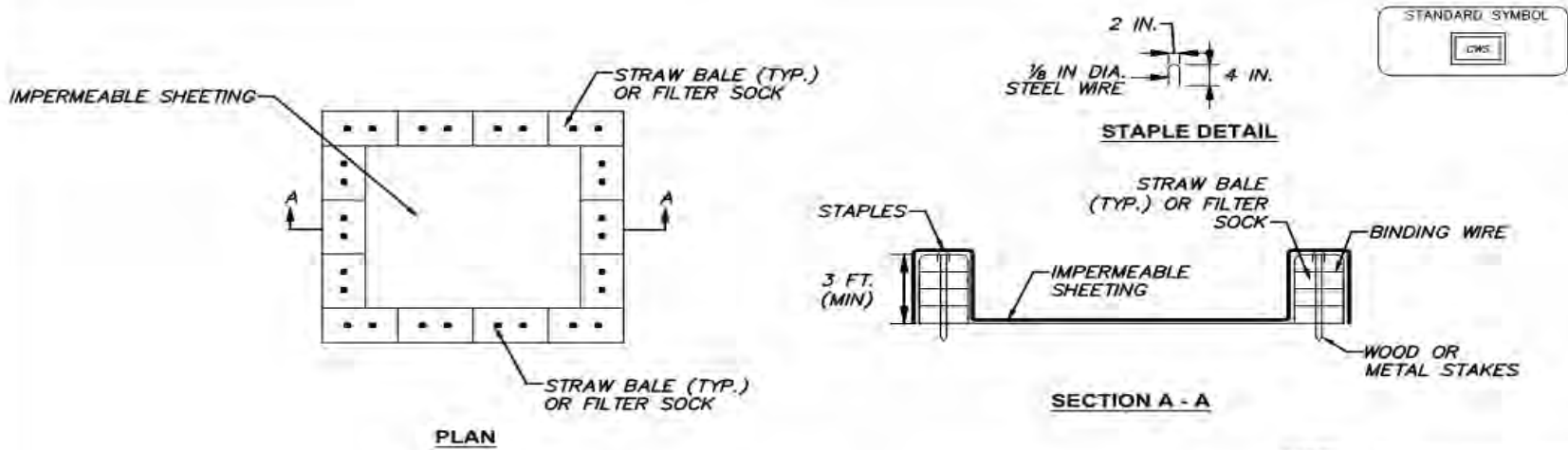
WASHOUT STRUCTURE WITH STRAW BALES OR FILTER SOCK
