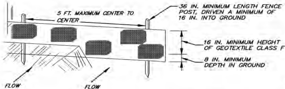
PERSPECTIVE VIEW
