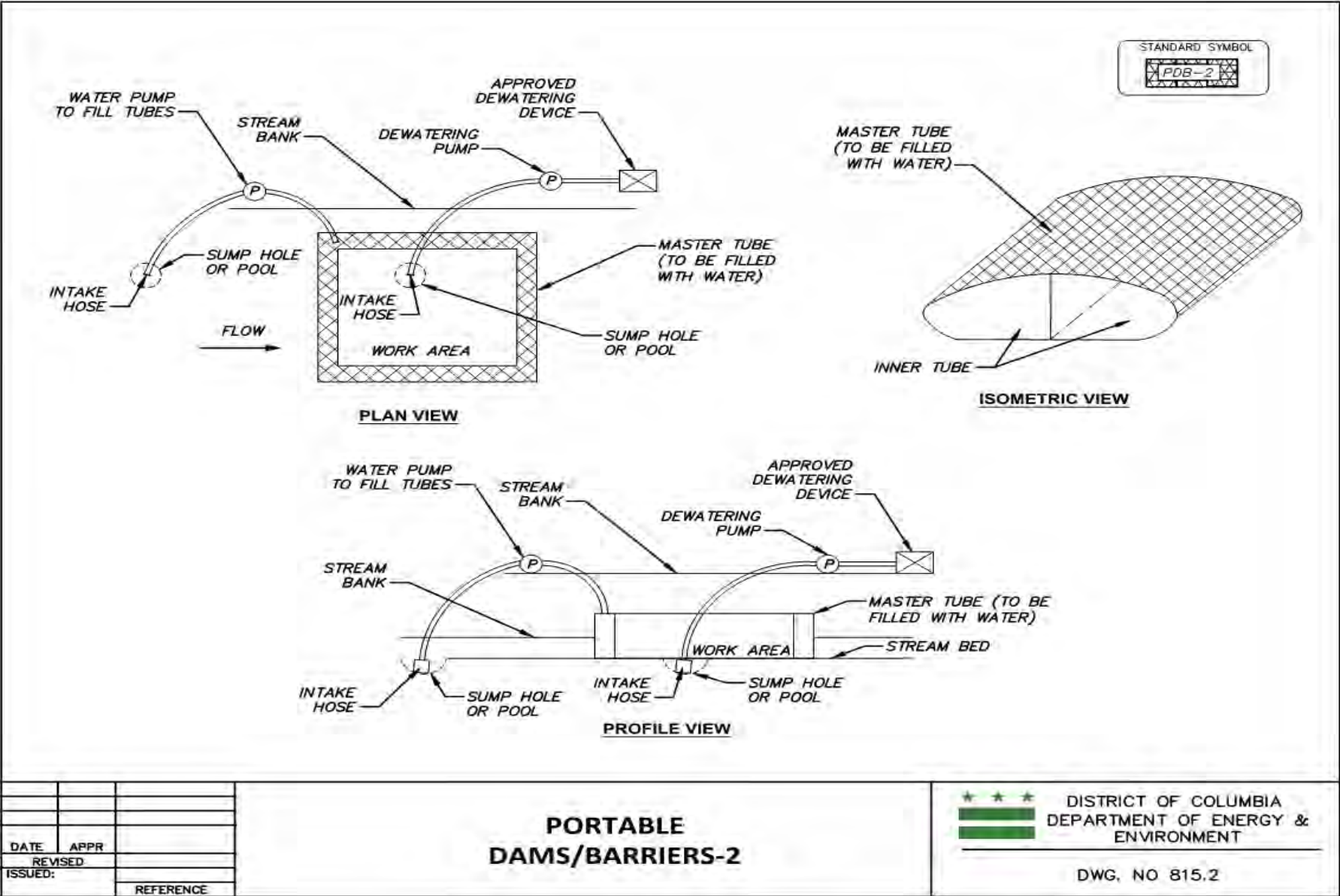
Detail 69 – 815.2 Portable Dams/Barriers - 2
