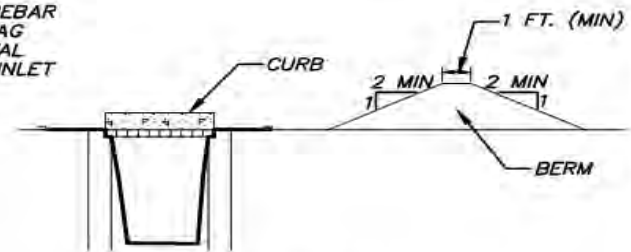
ELEVATION VIEW
