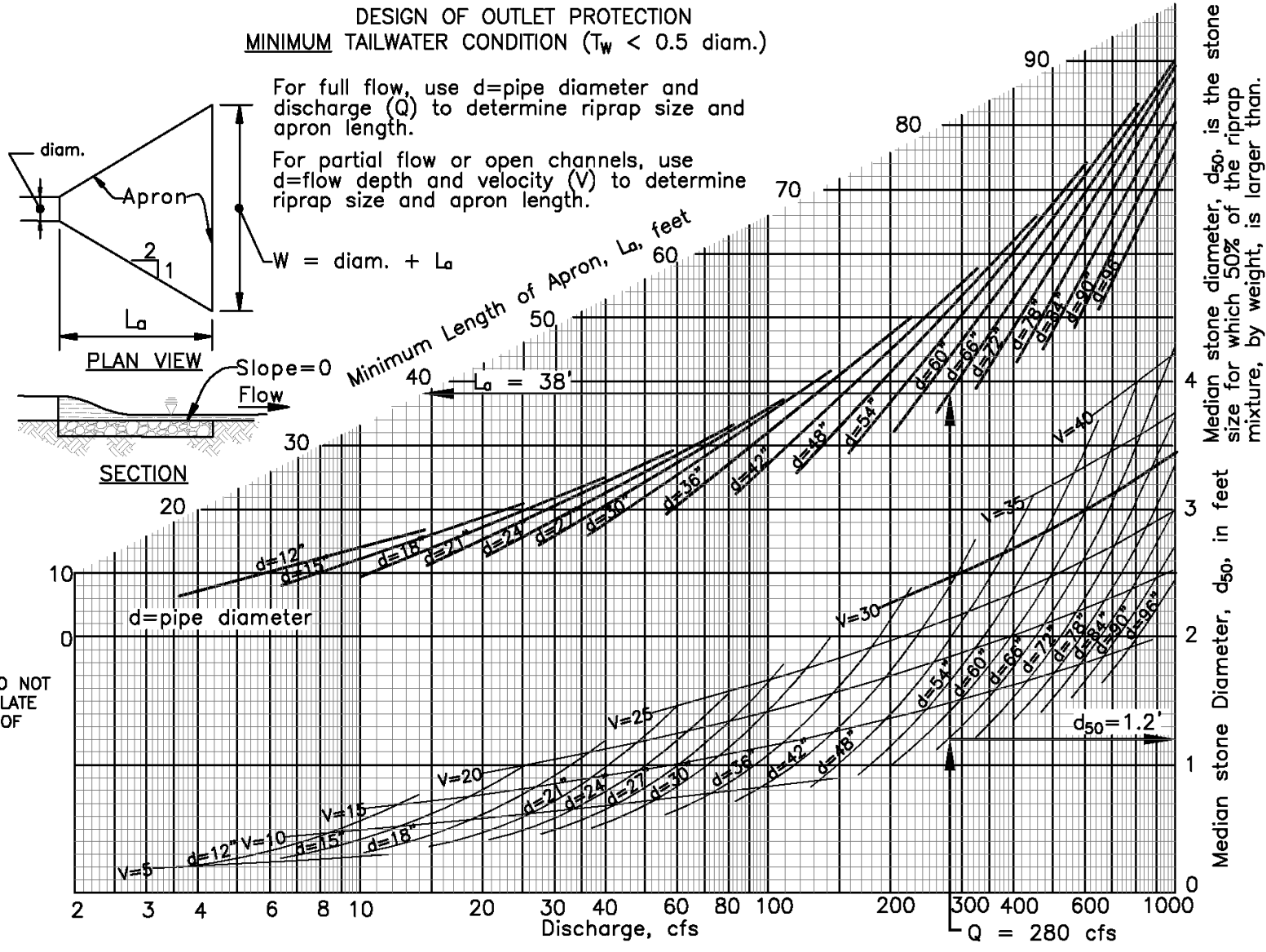
Figure 5.1 Design of outlet protection – minimum tailwater condition.
