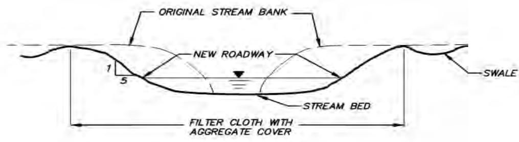
SECTION VIEW
