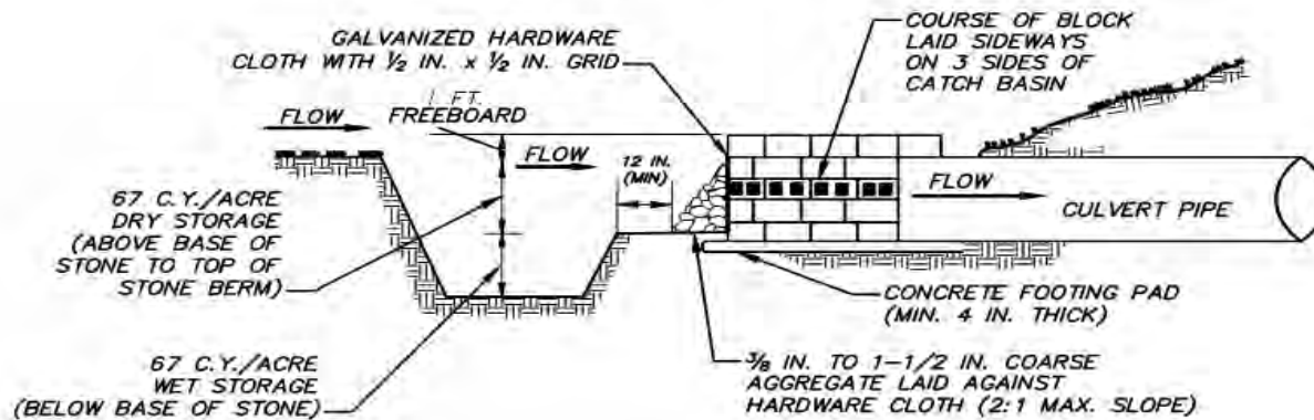
CROSS SECTION THROUGH "CATCH BASIN"
