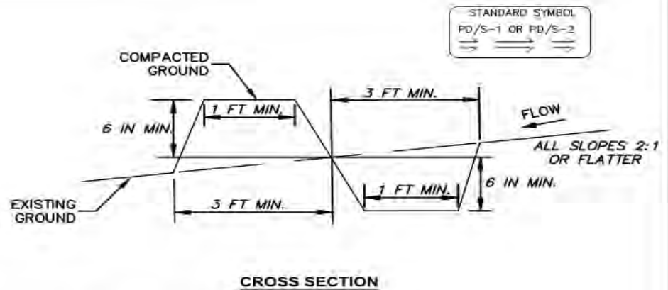
CROSS SECTION
