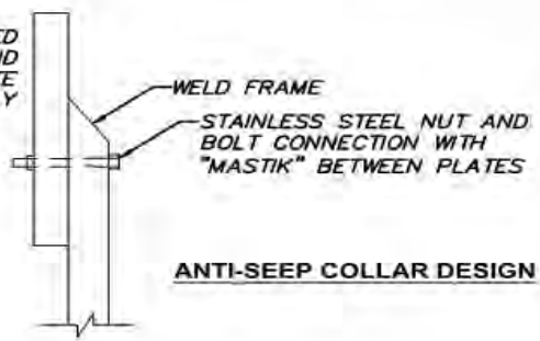
COLLAR WELDED IN PLACE ON BARREL SECTION
