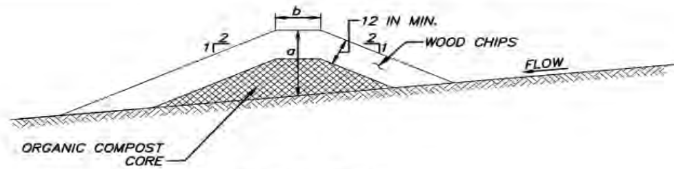
CROSS SECTION
