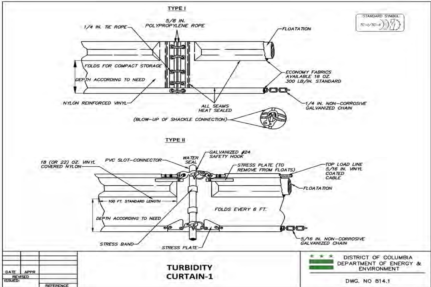
Detail 65 – 814.1 Turbidity Curtain - 1
