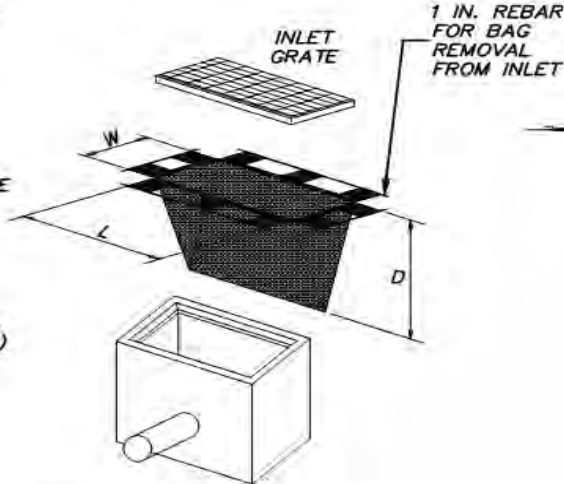
ISOMETRIC VIEW
