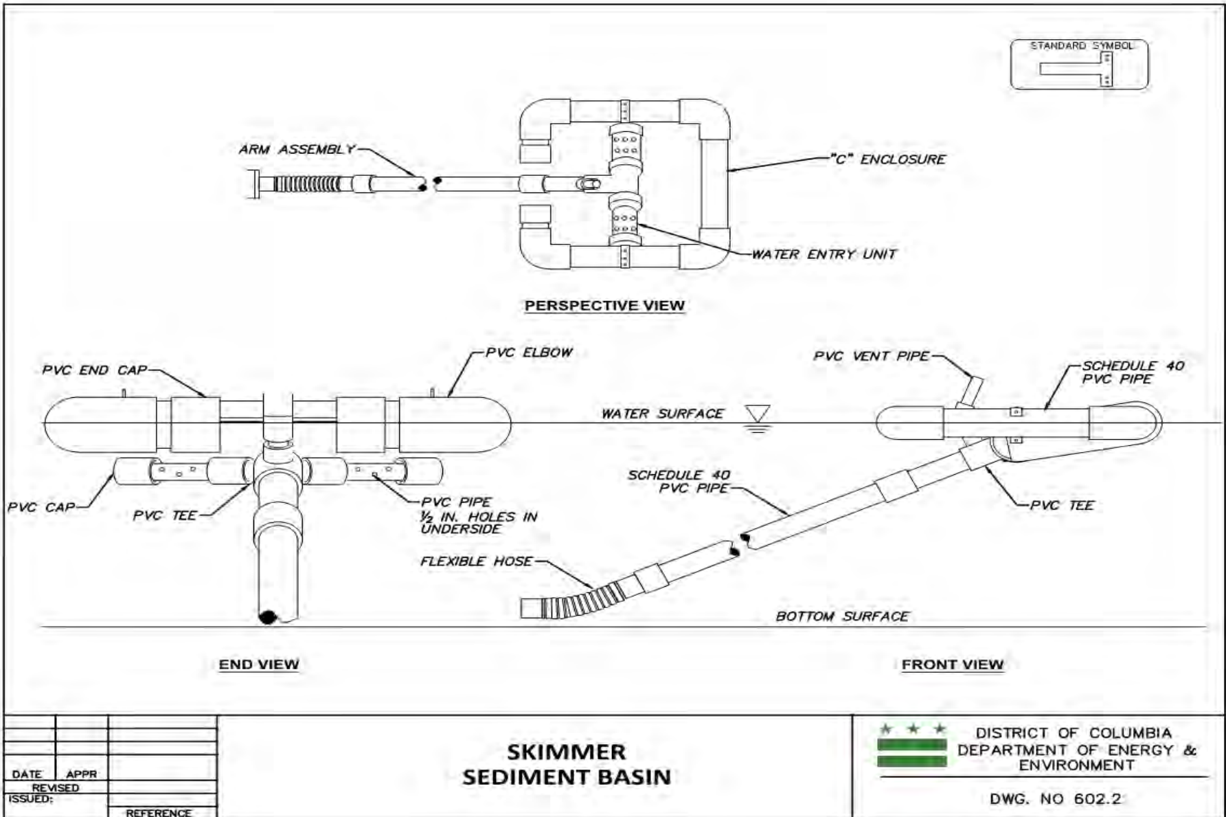
Detail 45 – 602.2 Skimmer
