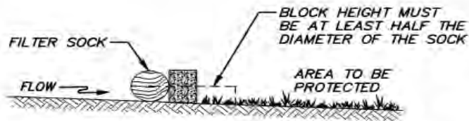
HARD SURFACE INSTALLATION SECTION
