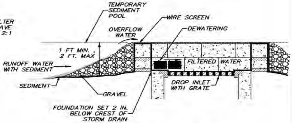
BLOCK AND GRAVEL SECTION A-A
