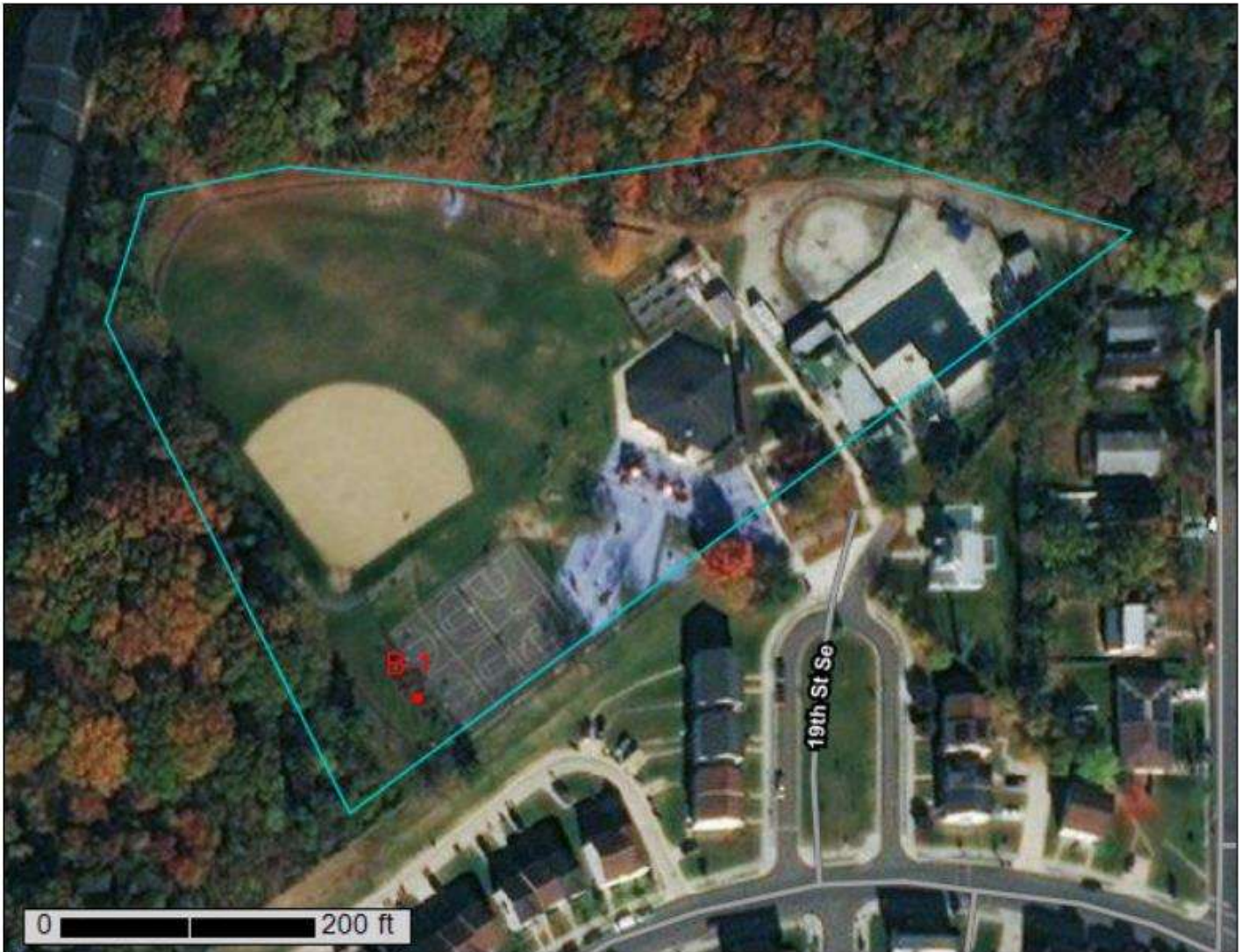
Figure 2 – Soil Boring Location
